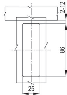
Panel Cutout
