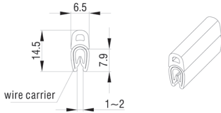
Sponge-rubber, black epdm gasket.
