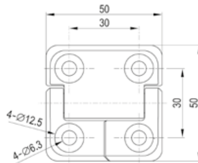
With Threaded Studs M6
